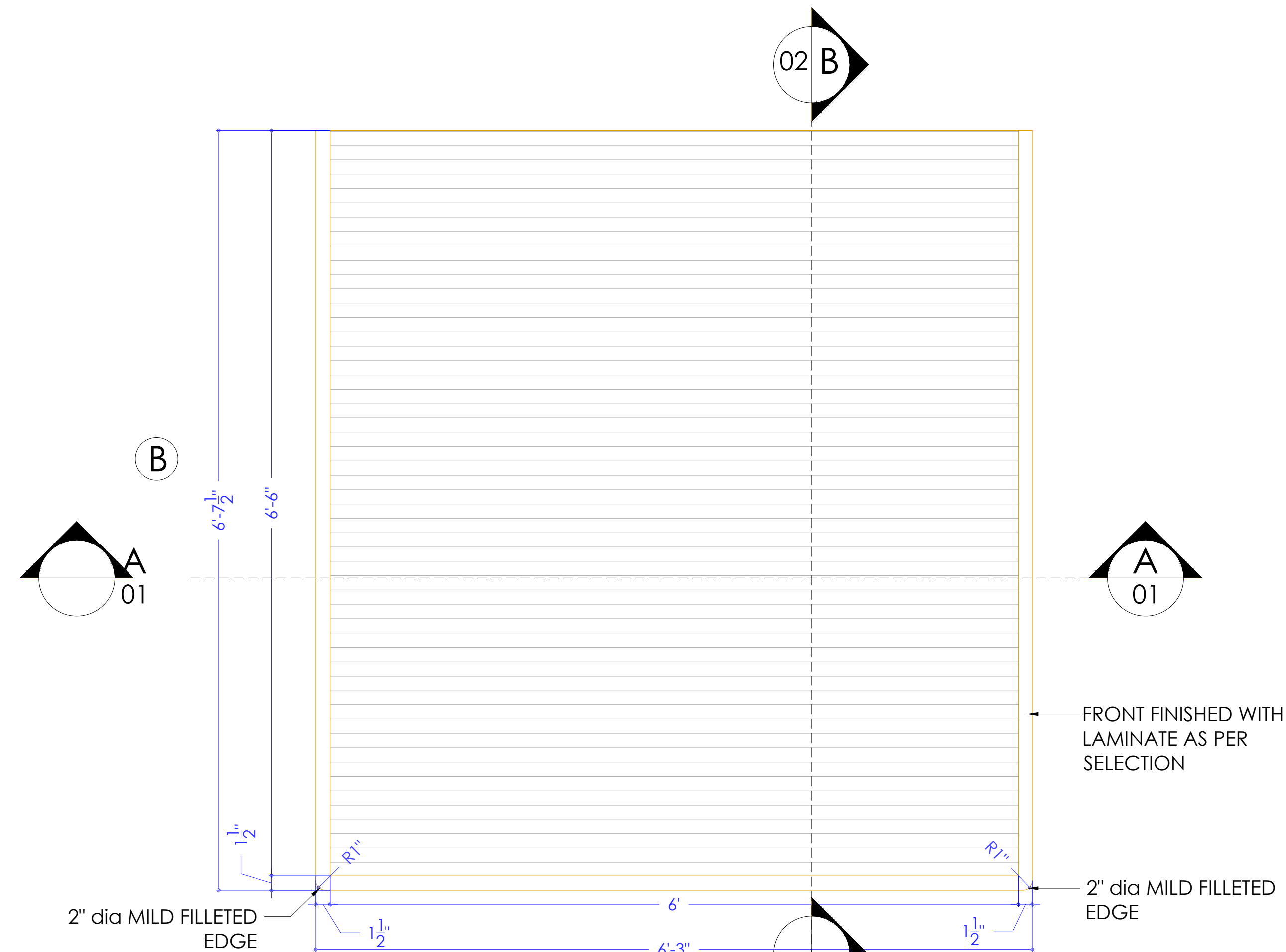
PLAN
