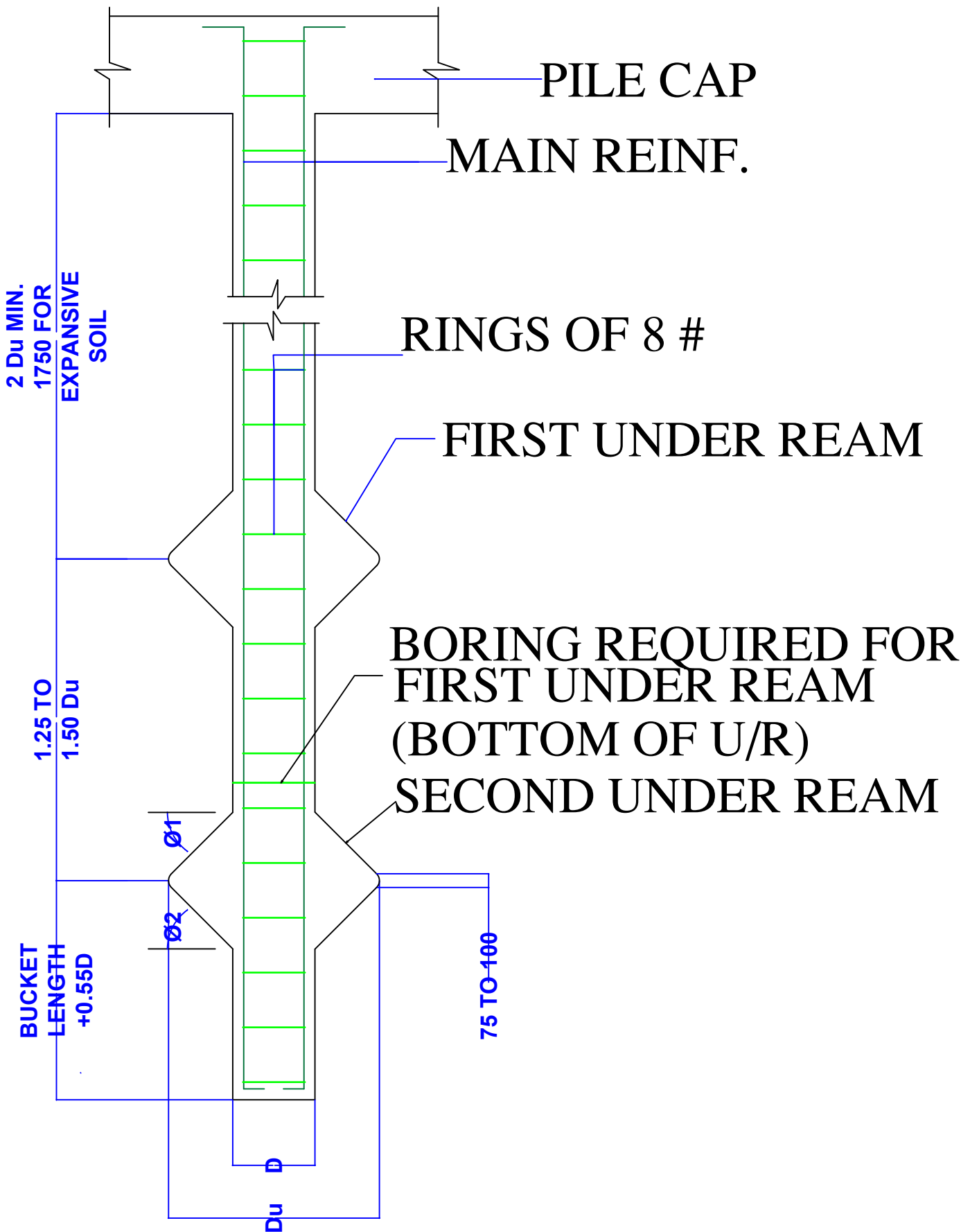
TYP. SKETCH OF DOUBLE UNDER REAMED PILE. (PILE-1)
