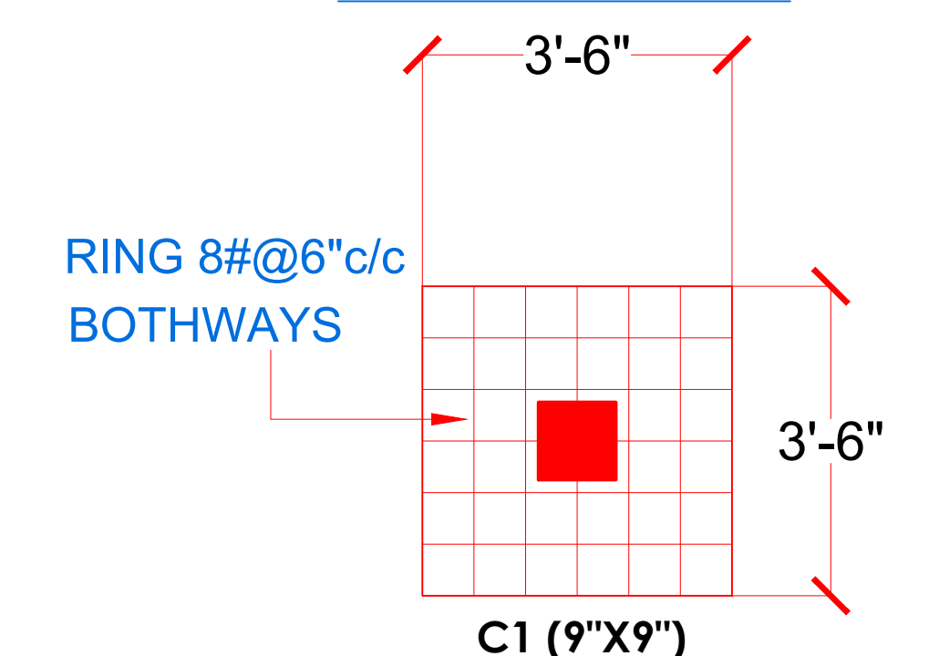
PLINTH BEAM
