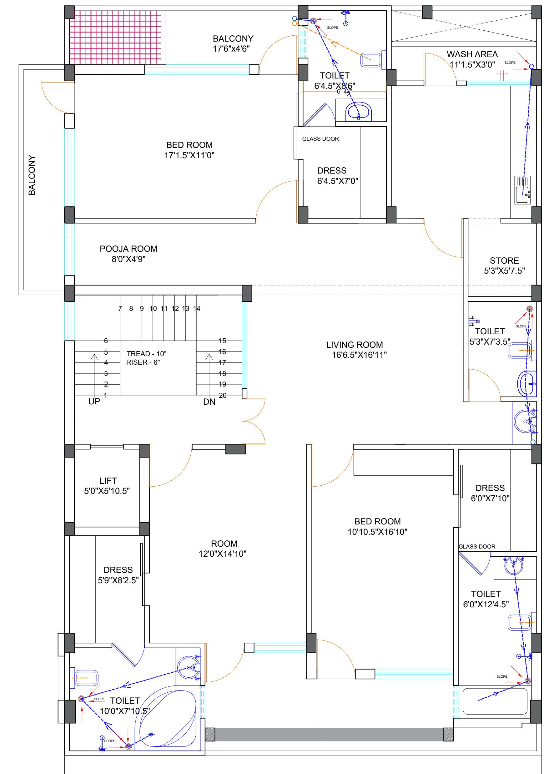
SECOND FL. SANITARY PLAN (PLOT 51)
