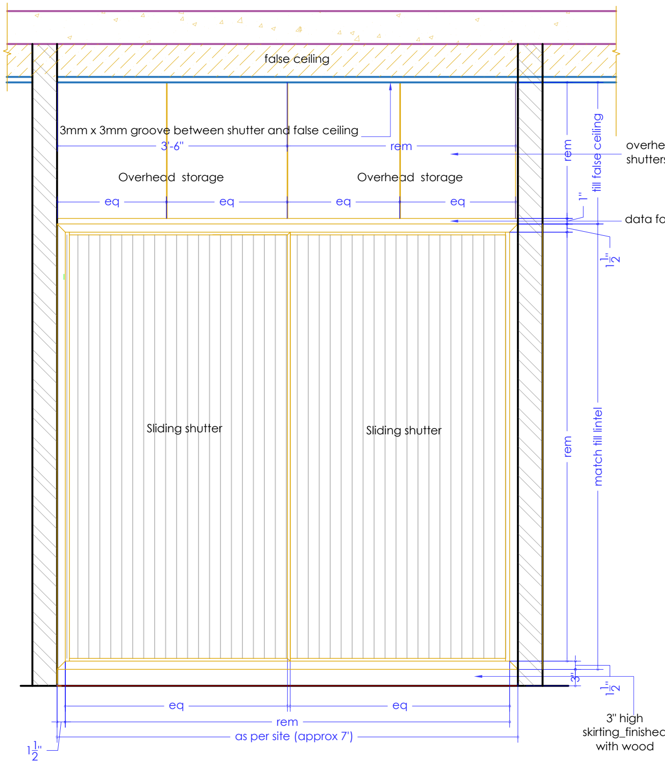
FRONT ELEVATION
