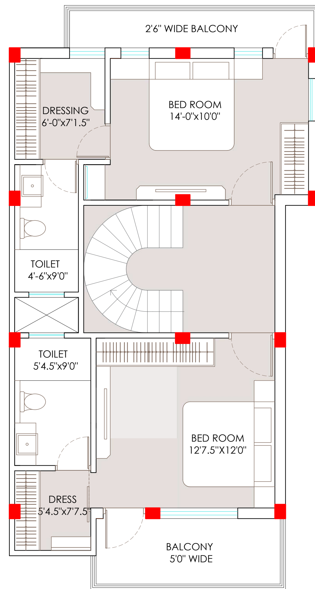
FIRST FLOOR.PLAN
