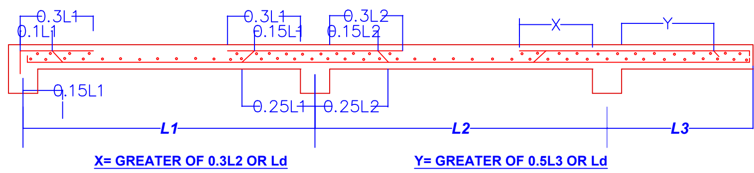
TYPICAL SKETCH OF SLAB
