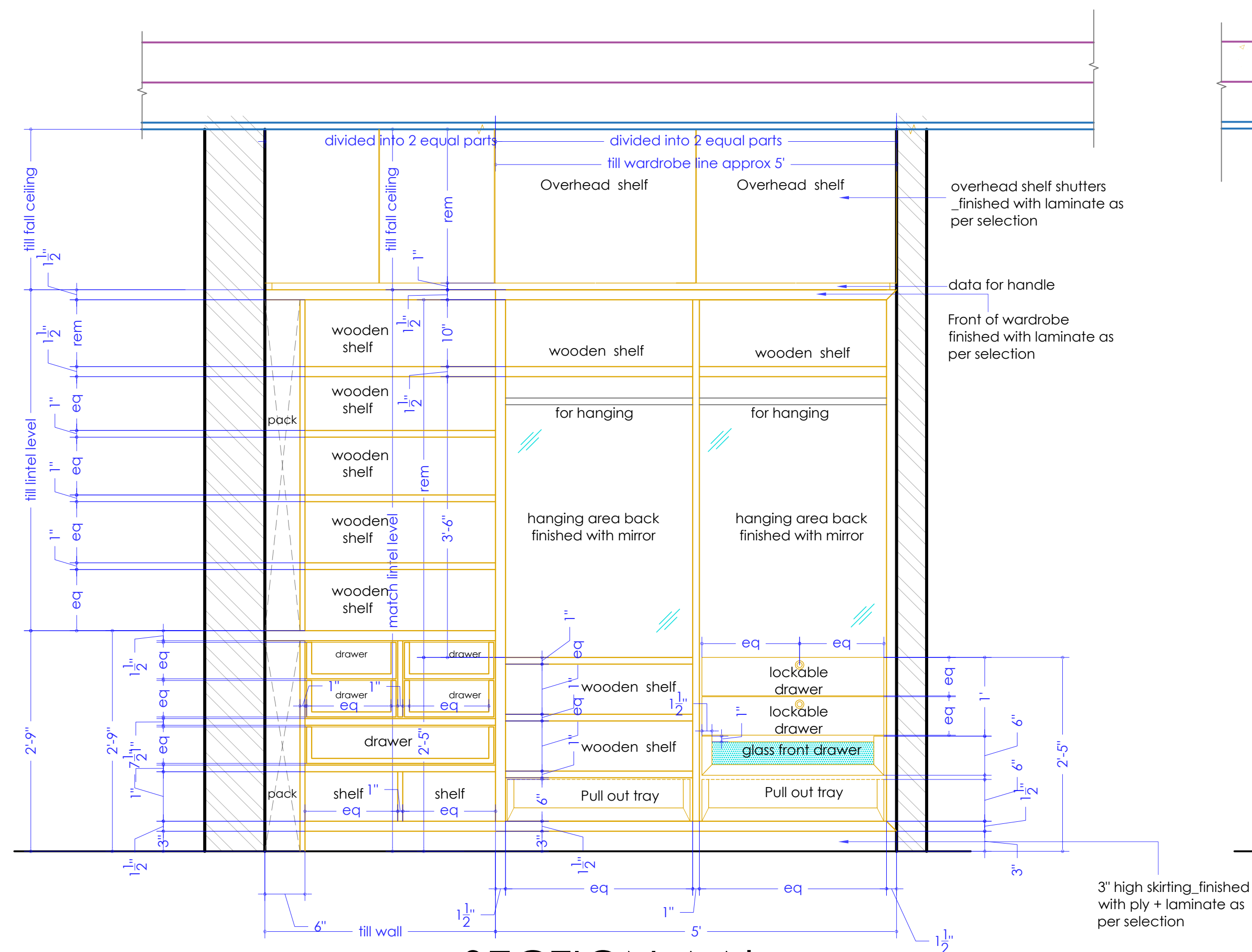
SECTION AA'
