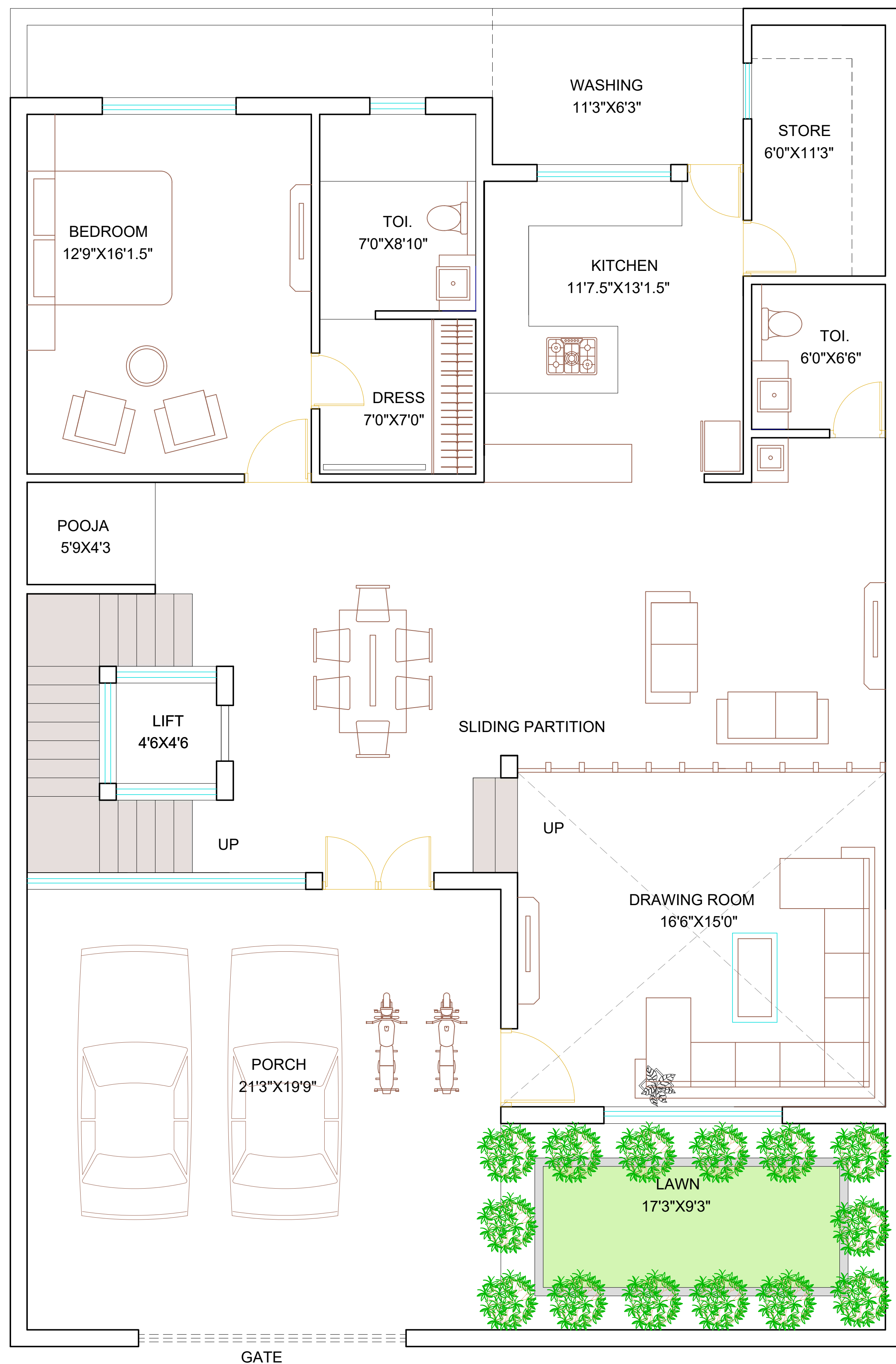
GROUND FLOOR
