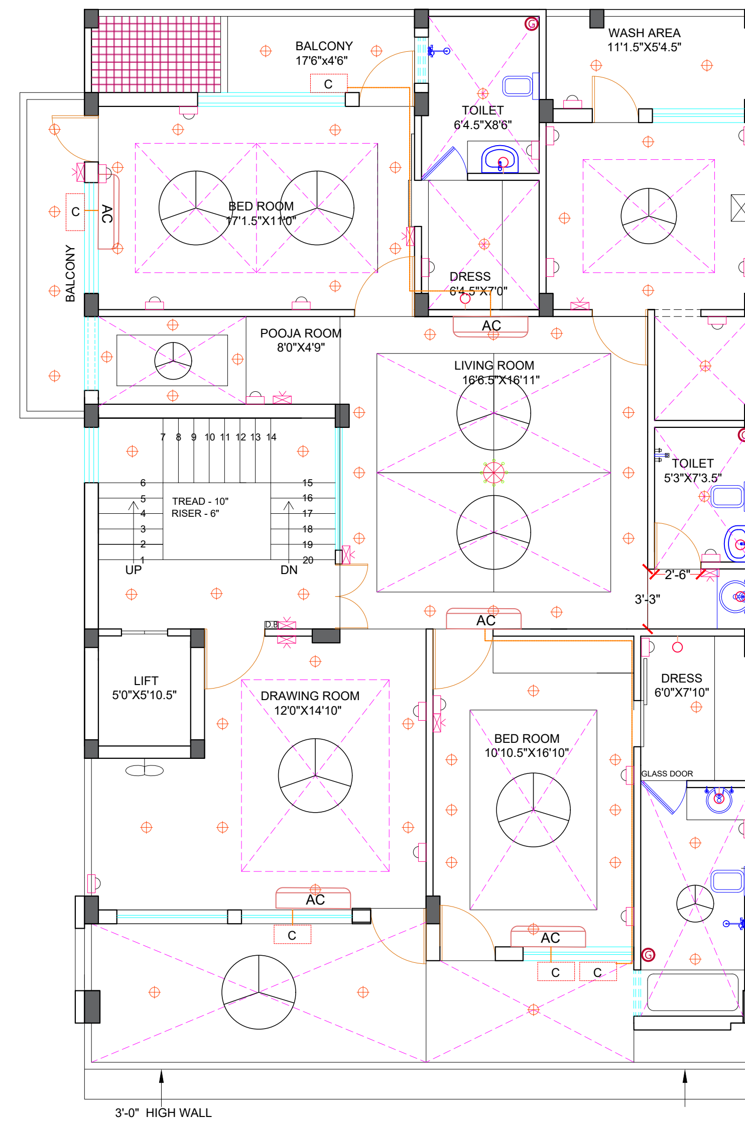
FIRST FL. LAYOUT ELECTRICAL PLAN (PLOT_51)
