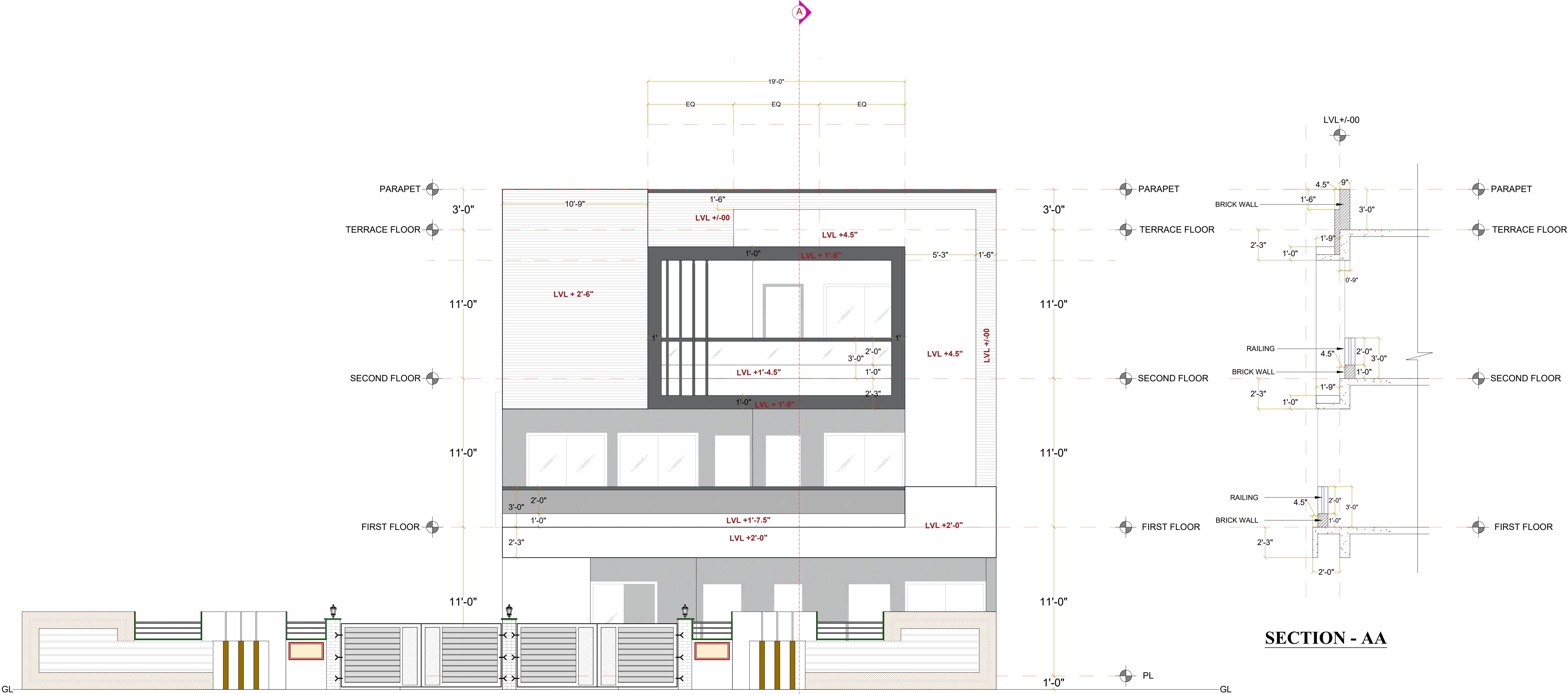
FRONT ELEVATION
