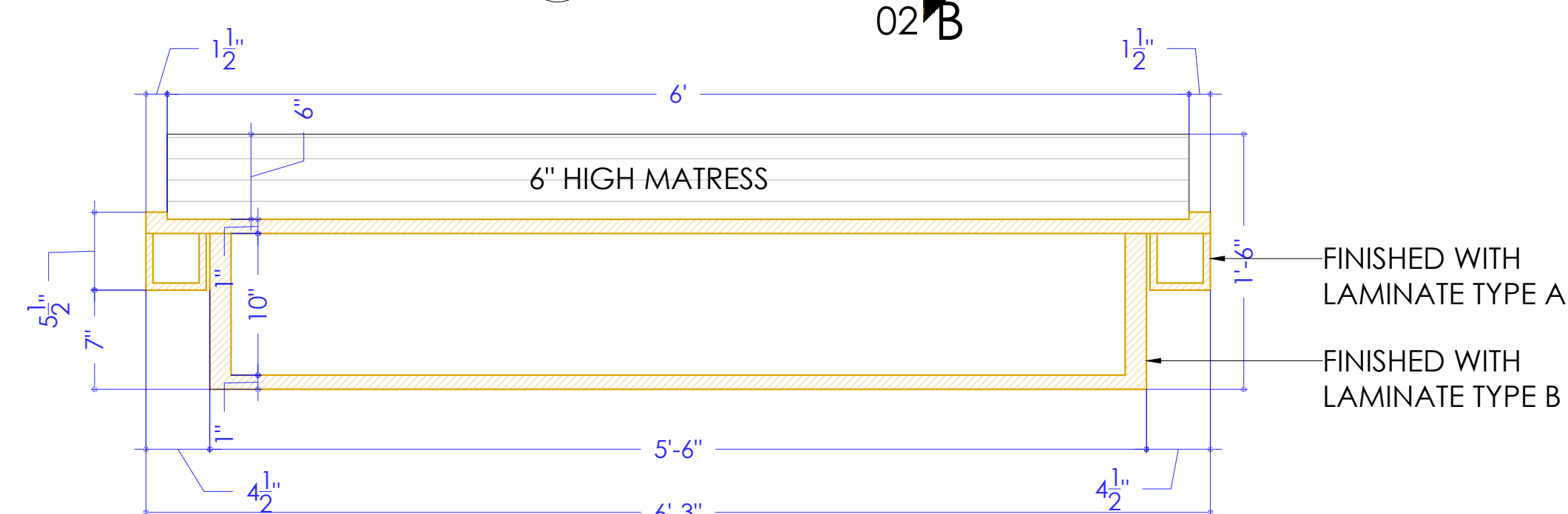
SECTION AA
