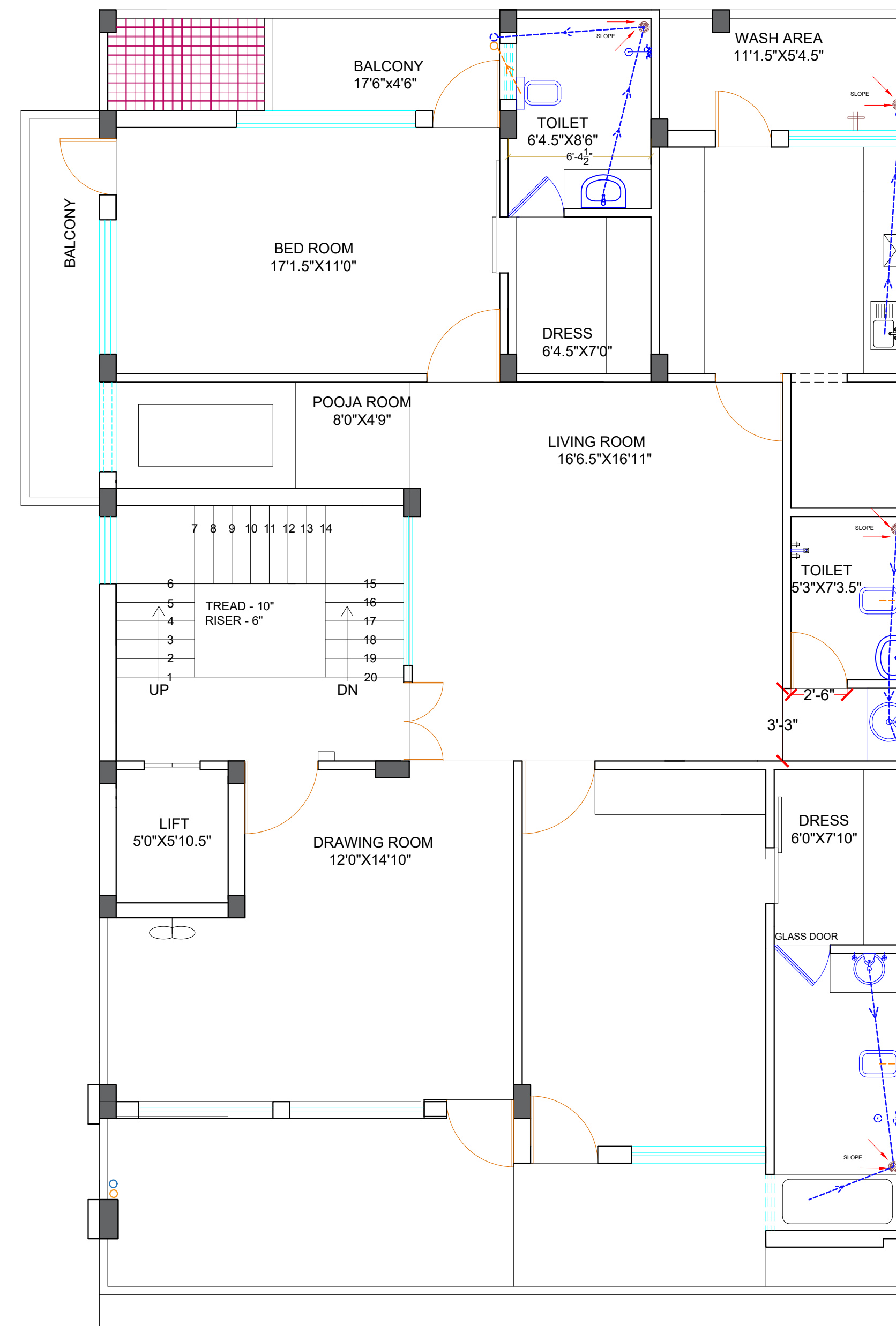
FIRST FL. SANITARY PLAN (PLOT 51)
