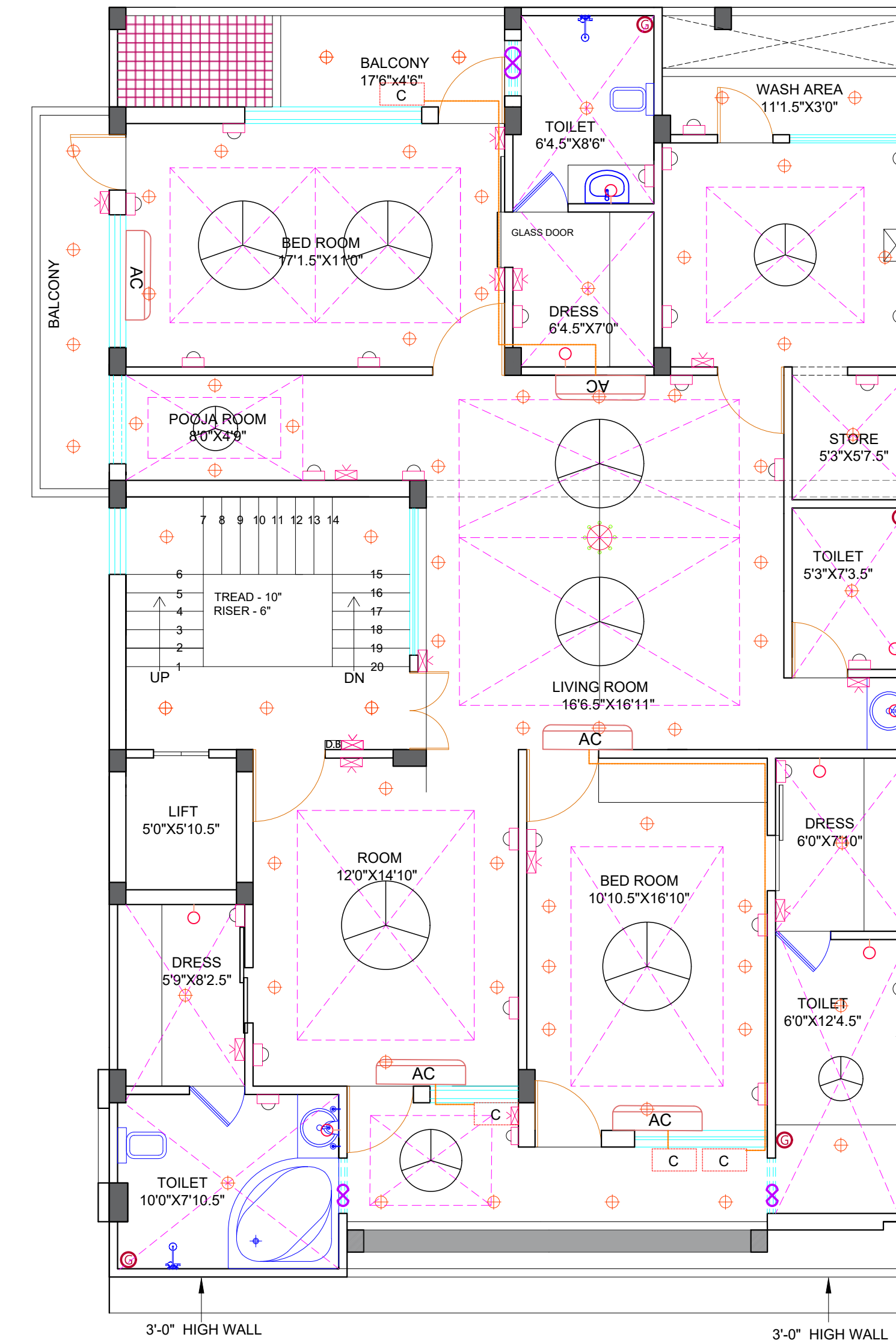
SECOND FL. ELECTRICAL LAYOUT PLAN(PLOT-51)
