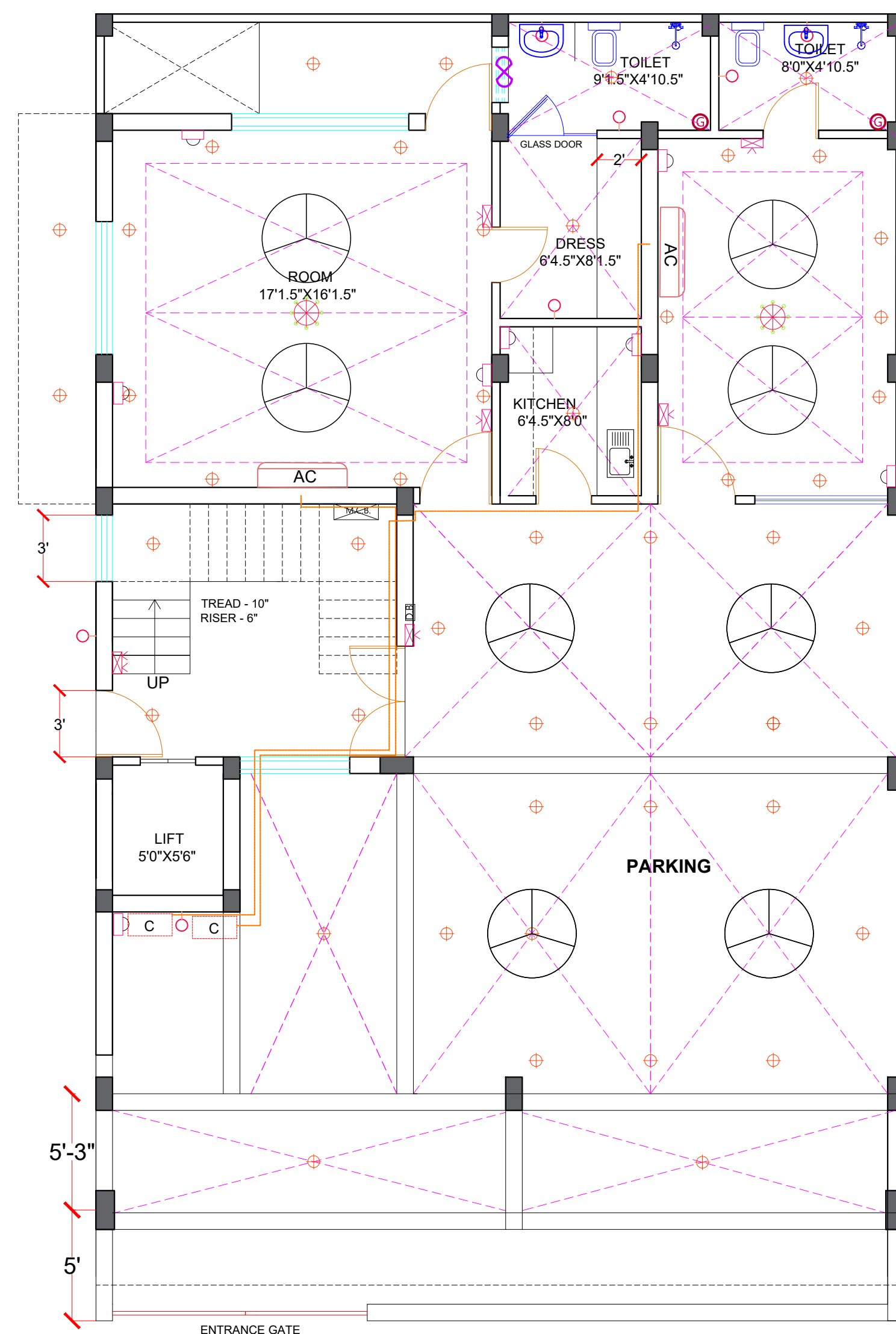
GROUND FL. LAYOUT ELECTRICAL PLAN_(PLOT 51)
