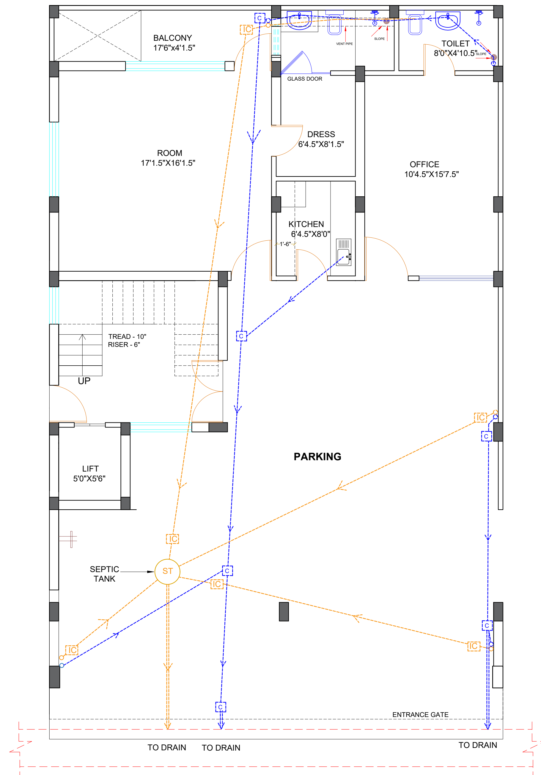
GROUND FL. SANITARY PLAN (PLOT 51)
