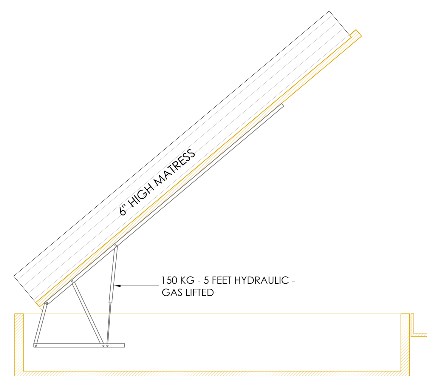
SECTION BB
