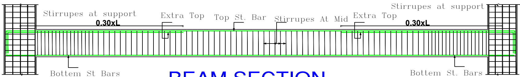
BEAM SECTION
