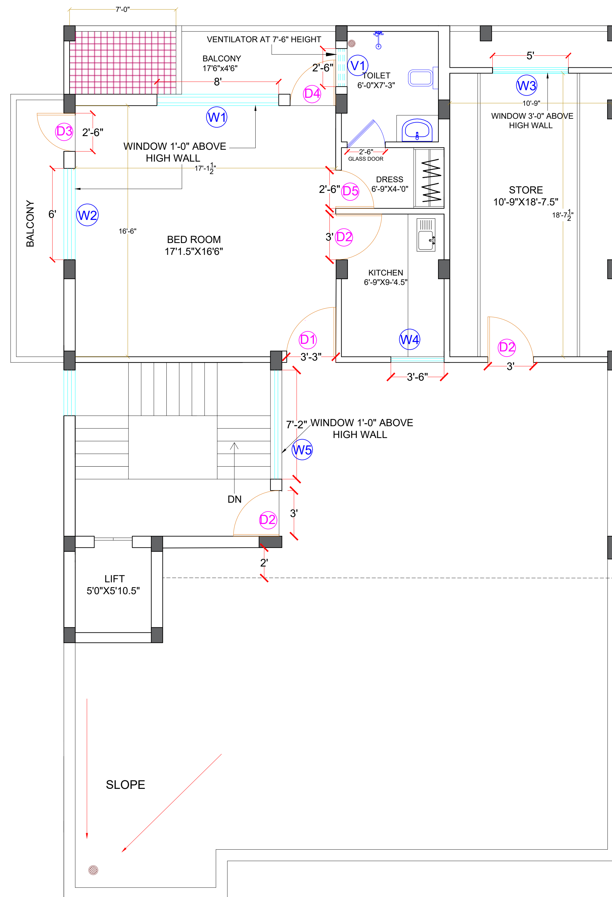
TERRACE FL. DOOR AND DETAILS(PLOT 51)
