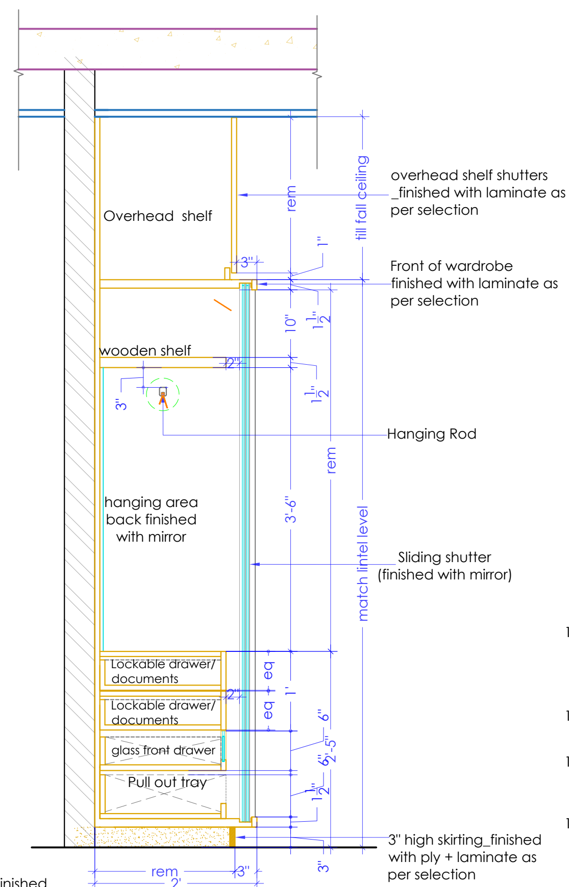
SECTION BB'
